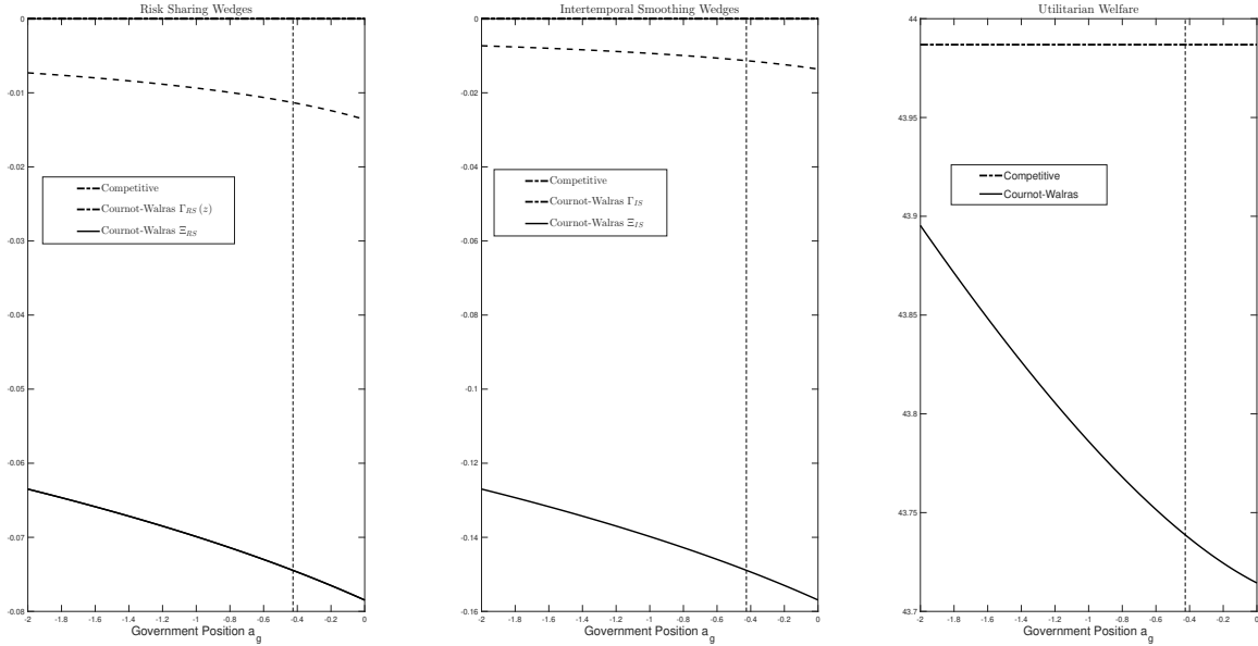
Figure 3: We plot the negative of our risk sharing gap, \Gamma_{RS}(z) , and intertemporal smoothing gap, \Gamma_{IS} , for comparison to the wedges of Davila and Schaab (2024) , \Xi_{RS} and \Xi_{IS} , in the left and middle panels, respectively, and utilitarian welfare in the right panel across government positions for the parameters in Table A.1
